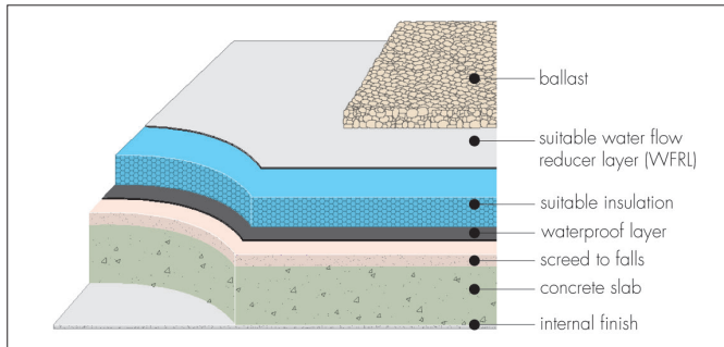
Typical inverted roof build up
